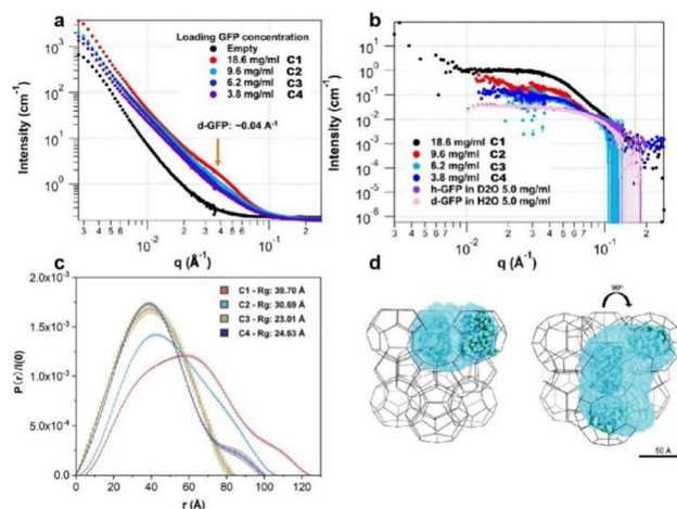
Fig. 14 (a) SANS spectra of d-GFP@MOF-919 with different protein loading content at the contrast matching point 50\% \text{ D}_2\text{O} . (b) Calculated spectra of d-GFP confined in MOF-919 after the subtraction of MOF scattering. (c) Pair distance distribution functions ( P(r) ) of d-GFP@MOF-919 with different protein loading content (C1–C4). (d) Ab initio structure reconstruction of C2 in the structure of MOF-919. The blue-shaded region is reconstructed using the scattering profile of C2, and the GFP atomic structure is overlaid as blue balls for comparison. Reproduced with permission from ref. 75.
