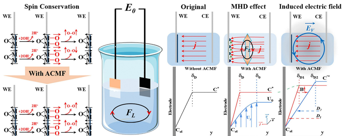
Fig. 13 Effect of AC magnetic field on magnetic catalyst in controlling the OER in an alkaline electrolyte. The diagram highlights how the AC magnetic field interacts with the catalyst surface and potentially enhances spin polarization and consequently modifies electron transfer dynamics. Figures are adopted from ref. 43 with permission from Elsevier B.V. © 2021.
