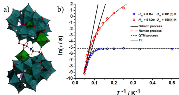
Fig. 8 The molecular structure (a) and magnetic relaxation plot (b) of [(\text{As}-\text{W}_9\text{O}_{33})_3\text{Dy}_2(\text{H}_2\text{O})_4\text{W}_4\text{O}_9(\text{H}_2\text{O})_2](\text{NH}_2(\text{CH}_2\text{PO}_3)_2)]^{33-} . Color code: cyan octahedron \{\text{W}_6\text{O}_6\} , green polyhedral Dy unit, red O, blue N, pink P, grey C, white H. Hydrogen atoms are omitted for clarity. Figure reprinted (adapted) with permission from ref. 136. Copyright (2017) American Chemical Society.
