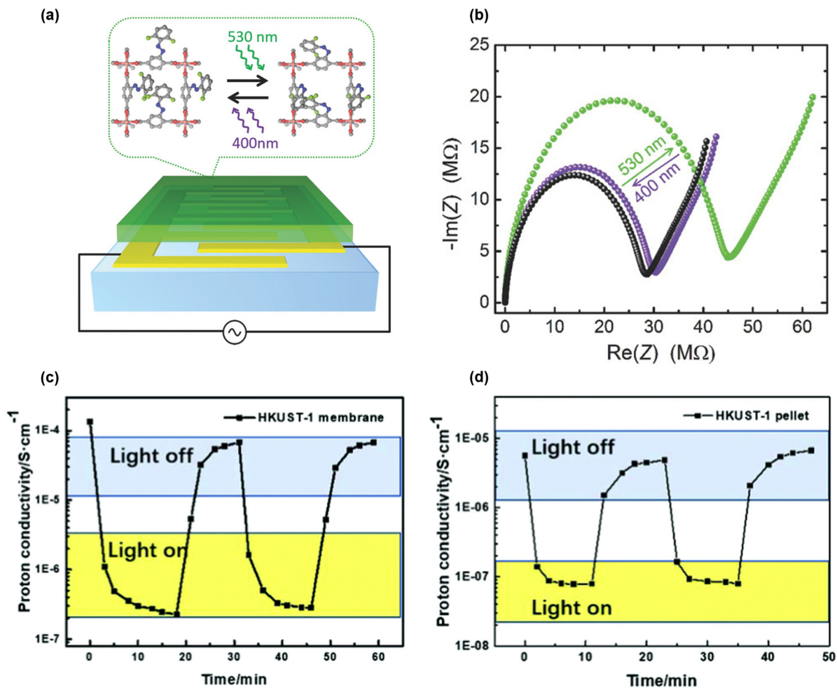
Fig. 10 (a) Schematization of surface mounted Cu 2 (F 2 AzoBDC) 2 (dabco) film: Cu 2 (F 2 AzoBDC) 2 (dabco) is the green layer on the interdigitated gold electrodes (yellow layer) on quartz substrate (light blue layer). Cu 2 (F 2 AzoBDC) 2 (dabco) structure viewed along the [001] direction. Black lines show the connection to the electric circuit and the impedance spectrometer. Representation of photoswitching between cis - and trans -fluorinated azobenzene side groups in Cu 2 (F 2 AzoBDC) 2 (dabco) when irradiated by green light (530 nm from trans to cis ) and with violet light (400 nm from cis to trans ). (b) Nyquist plot of the impedance of triazole@Cu 2 (F 2 AzoBDC) 2 (dabco). The black data is measured in the pristine sample ( trans ), green after irradiation with green light ( cis ), and violet after irradiation with violet light ( trans ). Reproduced with permission from ref. 92, Copyright 2018, Wiley, VCH. (c) and (d) Proton conductivity changes of the HKUST-1 (c) membrane and (d) pellet with and without light at 55 °C under 95% RH. Reproduced with permission from ref. 93, Copyright 2021, Royal Society of Chemistry.
