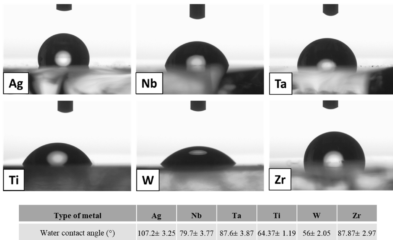
Fig. 4 Contact angle measurement of PVD-coated samples.
