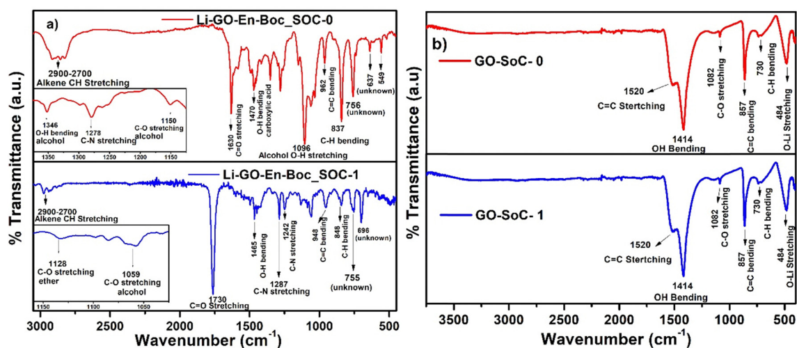
Fig. 11 Comparative FT-IR of (a) Li- \text{GO-EnBoc} and (b) \text{GO} at states-of-charge (SoC) \sim 0 (after the 1st discharge cycle) and 1 (after the 100th charge cycle).
