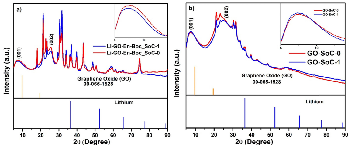
Fig. 10 XRD profiles at state of charge \sim 0 (after the 1st discharge cycle) and 1 (after the 100th charge cycle) for (a) Li- \text{GO-EnBoc} and (b) \text{GO} .
