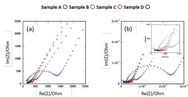
Fig. 6 AC impedance plots for samples after the 2 nd heating measured at (a) 30^{\circ}\text{C} and (b) -10^{\circ}\text{C} .
