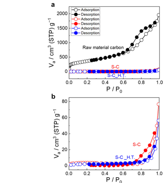
Fig. 3 (a) The N 2 adsorption/desorption isotherms of the raw material carbon, S-C and S-C_H.T. (b) The enlarged N 2 adsorption/desorption isotherms are also shown.
