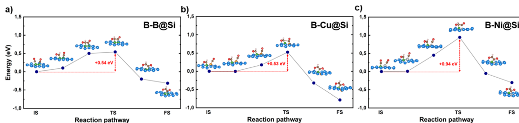
Fig. 4 The reaction path energy diagrams for the coupling step \text{CHO} - \text{CO}^* \rightarrow \text{OCHCO}^* on (a) B-B@Si, (b) B-Cu@Si and (c) B-Ni@Si. The insets show the atomic structures of initial state (IS), transition state (TS) and final state (FS). Red numbers indicate the activation energy barriers. Color code: B – green, Cu – orange, Ni – silver, Si – light blue, C – brown, O – red and H – light pink.
