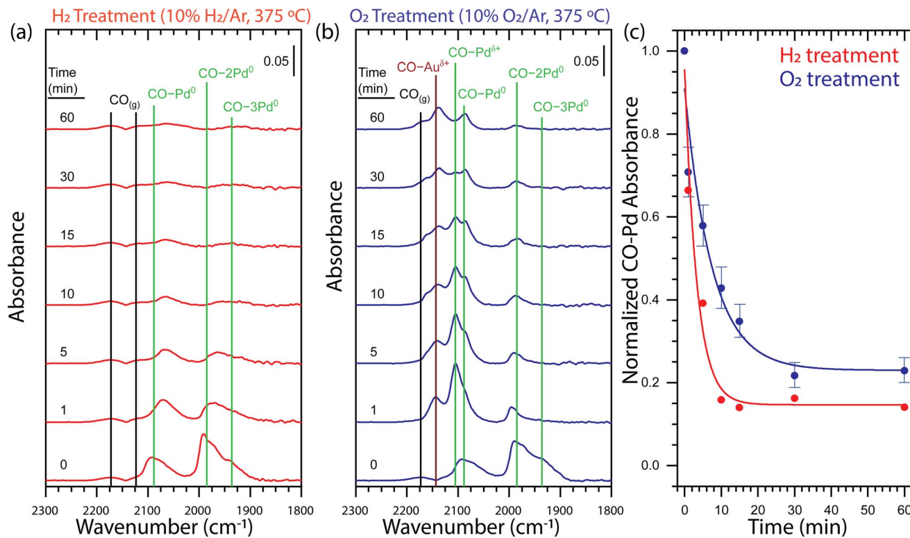
Fig. 3 Time-dependent DRIFT spectra for (a) \text{H}_2 and (b) \text{O}_2 treatments of core-shell Au-Pd/SiO 2 probed by CO adsorption demonstrate that the dissolution of Pd from the surface strongly depends on the gas environment. (c) Integrated CO-Pd bands of ex situ time-dependent DRIFT spectra for \text{H}_2 (red) and \text{O}_2 (blue) treatments of core-shell Au-Pd/SiO 2 normalized at t = 0 demonstrate that the \text{H}_2 treatment causes faster Pd dissolution and yields a lower Pd surface concentration. The guidelines through the \text{H}_2 and \text{O}_2 treatment integrated data are fitted with an exponential decay function. The error bars associated to the \text{O}_2 data points originate from the errors in the deconvolution of the CO-Pd peaks, as explained in Fig. S6.† The vibrational feature assignments are tabulated in Table S1† and additional evidence for the assignments are provided in Fig. S5.† Each spectrum panel denotes a 0.05 absorbance intensity legend. \text{H}_2 pretreatment: 5% \text{H}_2 in Ar, 250 °C, 45 min; \text{H}_2 treatment: 10% \text{H}_2 in Ar, 375 °C; \text{O}_2 treatment: 10% \text{O}_2 in Ar, 375 °C; CO adsorption conditions: 0.1% CO in Ar, 25 °C.
