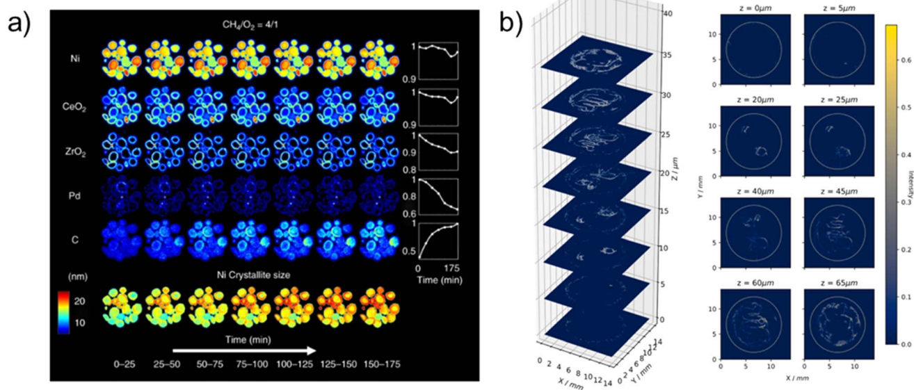
Fig. 7 (a) (Top): Synchrotron XRD-CT reconstruction showing chemical evolution of the complex Ni–Pd/CeO 2 –ZrO 2 /Al 2 O 3 catalyst during partial oxidation of methane. Phase distribution maps of Ni, CeO 2 , ZrO 2 , Pd and C are derived from Rietveld analysis. (Bottom): Crystallite size map of Ni, displaying the change in crystallite size, collected during partial oxidation of methane experiment. Reprinted under the terms of the Creative Commons Attribution 4.0 International (CC-BY 4.0) license, from Vamvakeros et al. , 118 Copyright 2018, The Author(s), published by Springer Nature. (b) XRD-CT scan of the MEA's Cu catalyst layer, demonstrating the versatile high energy X-ray transparent CO 2 electrolysis cell for operando WAXS/SAXS-CT measurements. The plotted intensity correspond to the surface oxide (Cu 2 O) XRD with one voxel resolution of 69.5 \mu\text{m} and the slice dimensions of 200 \times 200 voxels (13.9 \times 13.9 \text{mm}^2 ). Reprinted from Moss et al. , 86 Copyright 2023, with permission from Elsevier.
