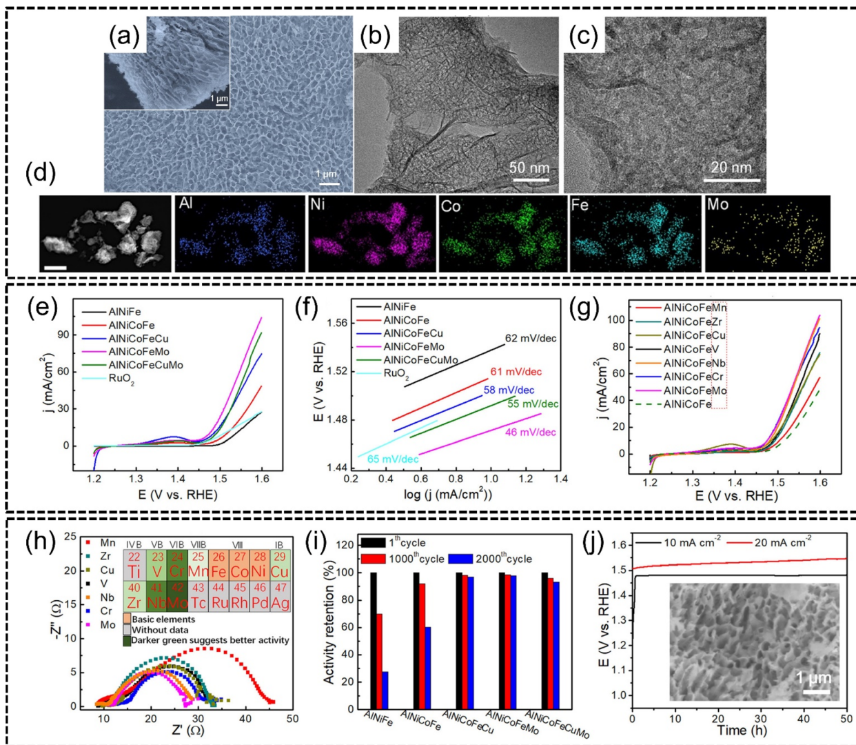
Fig. 13 The synthesis and OER performance of AlNiCoFeX ( X = \text{Mo}, \text{Nb}, \text{Cr} ) from the work of Qiu et al. Structural and morphological characterization, (a) plane-view and section view (inset) SEM images, (b) low magnification and (c) high magnification HRTEM images, and (d) STEM-EDX elemental mapping of AlNiCoFeMo nanoparticles. The scale is 150 nm. Electrochemical measurements (e), (g) LSV curves for the OER comparing different HEA combinations, (f) Tafel slopes, (h), EIS spectra with electrochemical enhancement effects of tested elements (inset), (i) potential change with time at 10 \text{ mA cm}^{-2} , and (j) potential-time graph with the SEM image of AlNiCoFeMo after 50 h of testing (inset). Reproduced with permission. 129 Copyright American Chemical Society 2019.
