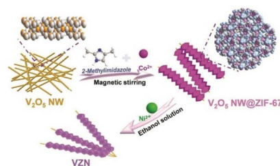
Fig. 3 Schematic illustration of the preparation of ZIF-67 on V_2O_5 NWs (VZN). (Panels) Reproduced with permission. 1 Copyright 2023, Wiley.
