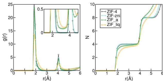
Fig. 2 Zn–N radial distribution function (left panel) and its integral (right panel) for ZIF-4, ZIF-zni, ZIF_a and ZIF_liq obtained by molecular dynamics simulations employing nb-ZIF-FF as a force field.
