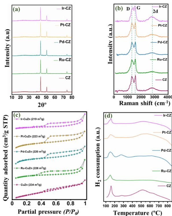
Fig. 2 (a) XRD pattern, (b) Raman spectrum, (c) \text{N}_2 physisorption isotherm and (d) TPR profile of CZ, Ru-CZ, Pd-CZ, Pt-CZ and Ir-CZ.
