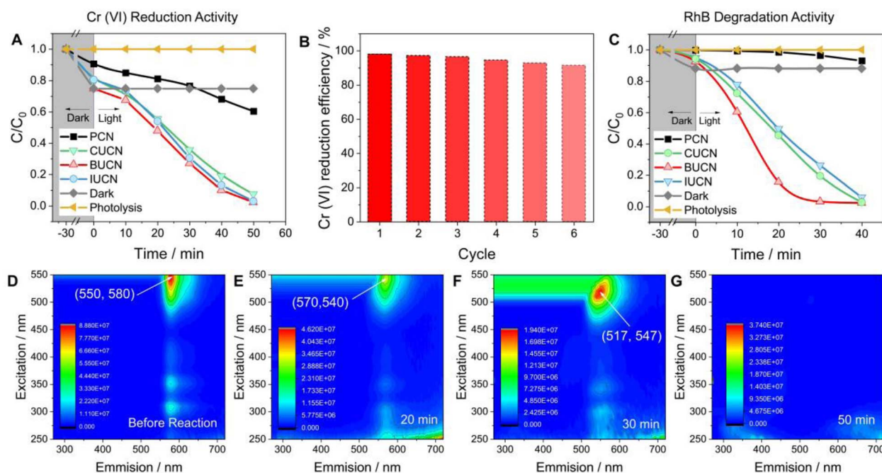
Fig. 5 Photocatalytic removal of aquatic pollutants: (A) photocatalytic Cr(vi) reduction performance of PCN and XUCN catalysts (reaction conditions: 20 mg of catalyst, 100 mL Cr(vi) solution of 10 mg L -1 ), (B) cyclic durability test of an optimized BUCN catalyst for Cr(vi) reduction during repetitive six cycles, (C) relative decrease in rhodamine B (RhB) concentration as a function of time over PCN and XUCN photocatalysts under visible light irradiation, and the corresponding 3D excitation-emission (3D EEM) matrix of (D) untreated RhB stock solution (before reaction), and photocatalytically treated RhB solution with a BUCN catalyst after (E) 20 min, (F) 30 min, and (G) 50 min of visible light irradiation, respectively.
