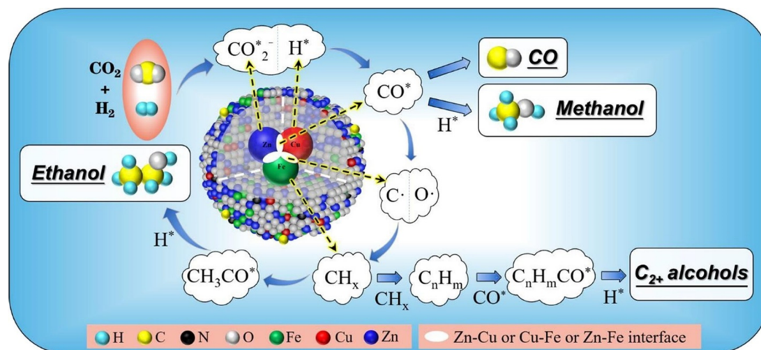
Fig. 8 The weak base of doped N promotes the generation of \text{CO}_2^* species through \text{CO}_2 activation, which is further regulated by the CuZnFe catalyst to form intermediates including \text{CO}^* , \text{CH}_x , and \text{HCOO}^* species to form higher alcohols through \text{CO}^* insertion into \text{C}_n\text{H}_m . Reprinted with permission from ref. 16. Copyright 2022 Elsevier.
