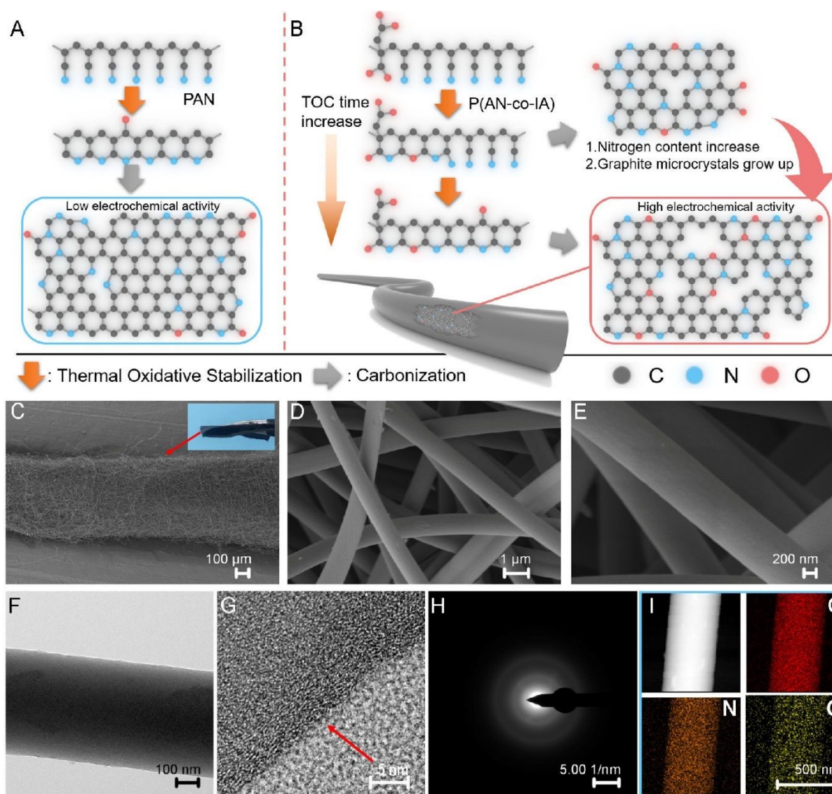
Figure 15: (a) Pictorial representation of carbonization procedure of PAN; (b) image of PAN copolymer carbonization. When the cyclization of precursor increases, pre-nitrogen content and material graphitization also increase. SEM image (c-e) carbonized CNF and image of piece of CNF. HRTEM image of CNF (f, g), (h) SAED image; (i) electron loss spectroscopy (EELS) elemental mapping. Reproduced with permission from [57] Copyright (2021) American Chemical Society.
