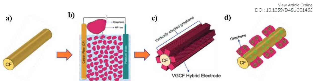
Figure 26: Pictorial representation of synthesis of VGCF electrode (a) CF substrate for electrophoretic deposition; (b) electrophoretic deposition with CF as negative electrode, Pt as positive electrode, and a bath consists of dispersion of graphene sheets in isopropyl alcohol with nickel nitrate hexahydrate; (c) VGCF hybrid after electrodeposition; (d) Pictorial representation of electron transport from graphene to CF. Reproduced with permission from [32] Copyright (2019) WILEY-VCH Verlag GmbH & Co. KGaA, Weinheim.
