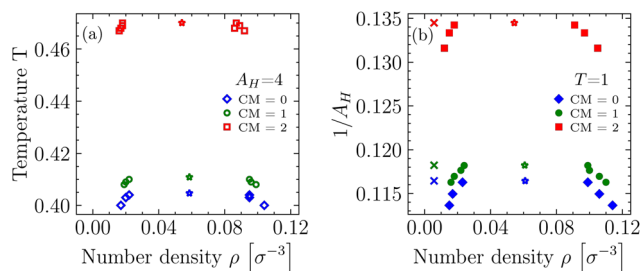
We utilize the obtained effective potentials in additional GCMC simulations, in which isotropic particles interact via the six critical U_{\text{eff}}(r) obtained by the previously described procedure. Subsequently, via the same protocol as described in Section 3 we determine critical temperatures T_c^{\text{iso}} for these systems and the obtained values are listed in Table 1. In the following sections of this paper these systems are referred to as “isotropic systems”. The obtained T_c^{\text{iso}} are approximately two to threefold higher as the corresponding T_c of the anisotropic models, pointing to a significant overrepresentation of attractions and/or underrepresentation of repulsions in U_{\text{eff}}(r) . An example are higher-order multi-body interactions not being present in U_{\text{eff}}(r) : it could be favorable for two CG molecules to form a low-energy dimer, which enters the effective potential. In the isotropic system three spheres can easily arrange to a trimer, with a threefold binding energy of the dimer, whereas three CG molecules can not easily arrange to a trimer with an equally low binding energy due to steric incompatibilities.
