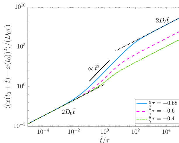
Fig. 4 Analytic result for the MSD in repulsive harmonic feedback potentials of varying strength (average taken over t_0 ). The repulsive feedback potential, pushing the particle away from its past position, leads to propulsion of the particle as indicated by the ballistic \propto \tilde{t}^2 regime of the MSD at intermediate times. Spatial diffusion additionally leads to changes in the angle between current and past position, causing the motion to become diffusive again on long time scales.
