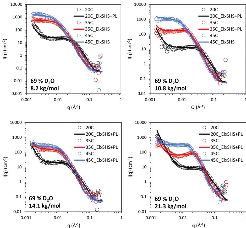
Fig. 6 SANS of 10 wt% BCS/3 wt% LAPONITE ® clay in 69% v/v D 2 O (in H 2 O), calculated to contrast match laponite. Lines represent a fit to the data shown as open circles, using the form factor inset. El: ellipsoid, SHS: sticky hard sphere, PL: power law. SANS data with error is included in Fig. S3–S6 (ESI † ).
