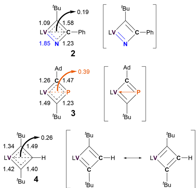
Fig. 6 Nalewajski-Mrozek bond orders of VCBDC scaffolds and most probable resonance structures of 2–4. L = dBDI 2- = ArNC(CH 3 )CHC(CH 2 )NAr, Ar = 2,6- t Pr 2 C 6 H 3 .
