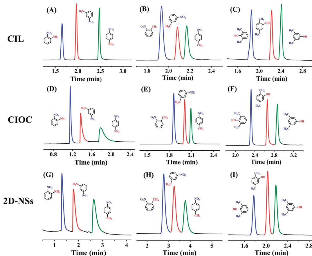
Fig. 4 Gas chromatograms of positional isomers on CIL, ClOC and 2D-NSs coated capillary columns: nitroaniline (A, D, and G), nitrotoluene (B, E, and H), and dimethylphenol (C, F, and I). Oven program: 100–170 °C at 30 °C min -1 for (A), 50–150 °C at 30 °C min -1 for (B), 70–150 °C at 20 °C min -1 for (C), 120–180 °C at 50 °C min -1 for (D), 80–140 °C at 30 °C min -1 for (E), 100–150 °C at 20 °C min -1 for (F, and G), 90–160 °C at 20 °C min -1 for (H), and 120–150 °C at 20 °C min -1 for (I). Flow rate: 3.0 mL min -1 for (A, and B); 2.0 mL min -1 for (C, E, and G); 4.0 mL min -1 for (D); 1.5 mL min -1 for (F); 0.8 mL min -1 for (H); and 1.0 mL min -1 for (I).
