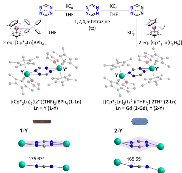
Fig. 1 Top: Synthetic pathways for the isolation of the \text{tz}^{\cdot-} -bridged ( 1\text{-Ln} ) and \text{tz}^{2-} -bridged ( 2\text{-Ln} ) dinuclear complexes. Middle: Molecular structures of 1\text{-Y} and 2\text{-Y} , where partial labelling and omission of H-atoms, disordered conformers, THF lattice solvents and the \text{BPh}_4^- counter ion for 1\text{-Y} have been employed for clarity. Images of the respective single crystals (dark red for 1\text{-Y} ; violet for 2\text{-Y} ) under an optical microscope are given for each complex. Bottom: magnification of the \text{Y}_2\text{-tz} core, highlighting the significantly increased tilting of the \text{tz}^{2-} ring in 2\text{-Y} compared to \text{tz}^{\cdot-} in 1\text{-Y} .
