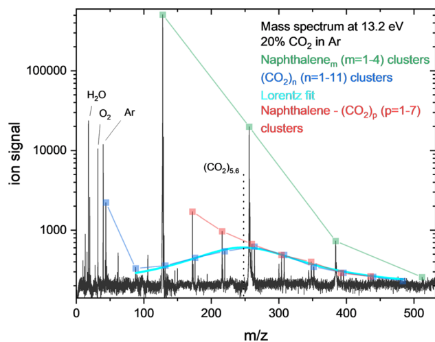
Fig. 4 Mass spectra at 13.2 eV photon energy (black) where least fragmentation of pure \text{CO}_2 clusters is expected (see Fig. 3). Indicated are the pure \text{CO}_2 clusters (dark blue), the naphthalene clusters (green) and the naphthalene- \text{CO}_2 clusters (red). A Lorentz fit of the pure \text{CO}_2 cluster size distribution (light blue), not including the monomer, indicates a mean cluster size of 5.6 \text{CO}_2 units.
