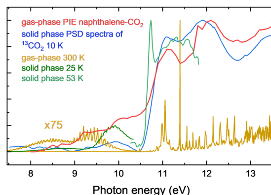
Fig. 5 Comparison of the PIE curve of naphthalene- \text{CO}_2 with solid phase photon-stimulated desorption (PSD) spectrum of ^{13}\text{CO}_2 , 20 \text{CO}_2 gas-phase spectrum 39 and \text{CO}_2 solid phase absorption spectra. 40–42
