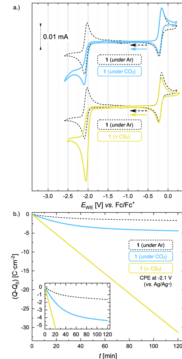
Fig. 5 (a) CV of 1 (1 mM) under Ar (black, dashed line), under \text{CO}_2 (light blue, solid line), and in the presence of \text{CS}_2 (1 equiv.) in \text{TBAPF}_6/\text{MeCN} (0.1 M) at a scan rate \nu = 20 \text{ mV s}^{-1} . (b) Passed charge ( Q - Q_0 ) vs. time of CPE for 2 hours of 1 (5 mM) under Ar (black, dashed line), under \text{CO}_2 (light blue, solid line) and in the presence of excess \text{CS}_2 (56 equiv.).
