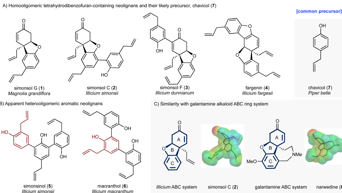
Fig. 1 Structures of Illicium -derived neolignan natural products.
