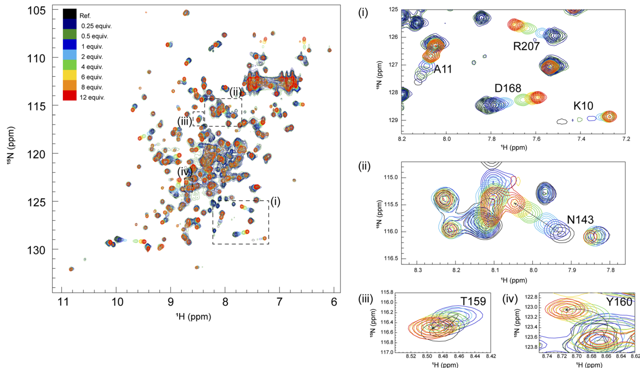
Fig. 1 Overlays of 2D ^1\text{H} - ^{15}\text{N} HSQC spectra from multipoint titrations of ^{15}\text{N} -labelled GRB2 with SOS1-S4 PRM (VPPVPVPPRRR). The PRM concentration was increased stepwise (the protein: PRM molar ratio of 1 : 0.25, 1 : 0.5, 1 : 1, 1 : 2, 1 : 4, 1 : 6, 1 : 8, and 1 : 12). In this figure, the colour codes of ^1\text{H} - ^{15}\text{N} correlation cross-peaks at each titration point, showing the molar ratio of GRB2: SOS1-S4, are as follows: black (1 : 0); dark blue (1 : 0.25); dark green (1 : 0.5); blue (1 : 1); cyan (1 : 2); green (1 : 4); yellow (1 : 6); orange (1 : 8); red (1 : 12). Cross-peaks that showed large chemical shift changes are annotated.
