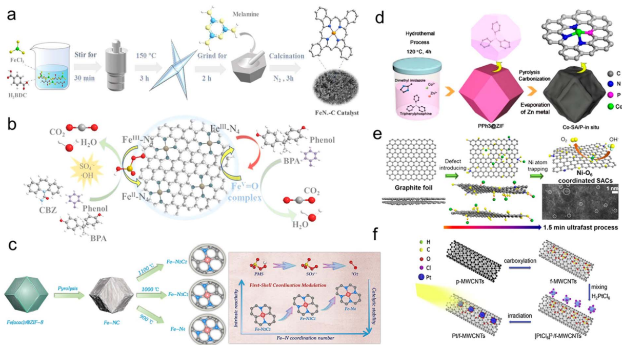
Fig. 6 (a) The preparation of \text{FeN}_x\text{-C} catalysts (Fe SACs); (b) the proposed mechanism of \text{FeN}_x\text{-C}/\text{PMS} system; 86 Copyright 2021 American Chemical Society. (c) The synthesis strategy of \text{FeN}_x catalysts based on pyrolysis temperature and the relationship between Fe–N coordination number and the intrinsic reactivity; 150 Copyright © 2023 American Chemical Society. (d) The fabrication process of Co-SA/P catalysts; 153 Copyright © 2020 American Chemical Society. (e) Schematic of the synthesis process for Ni SACs; 161 Copyright © 2020 American Chemical Society. (f) The preparation strategy of Pt/f-MWCNTs; 162 figures have been adapted from ref. 86, 150, 153, 161 and 162 with permissions from the American Chemical Society, Copyright 2022, American Chemical Society, Copyright 2023, American Chemical Society, Copyright 2020, American Chemical Society, Copyright 2020 and Elsevier B.V. Copyright 2019, respectively.
