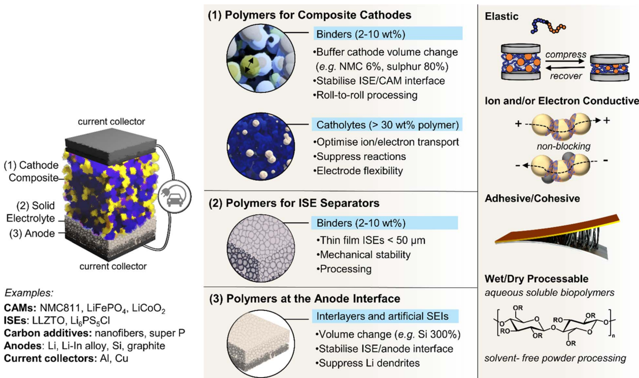
Fig. 5 Roles of polymers in solid-state batteries with inorganic solid electrolytes (ISEs). From the left: solid-state cell with thick composite cathode comprised of cathode active material (CAM), ISE, carbon additive and polymer binder in \sim 70 : 23 : 2 : 5 wt% ratio (1), thin-film ISE layer (2) and Li or Li-rich metal foil anode (3). Polymers play roles as functional binders and coatings, protective interlayers and interphases and active electrode material. SEI, solid electrolyte interphase. Elastic polymers are required to buffer electrode volume changes and intrinsic ionic and/or electron polymer conductivities to facilitate ion/electron pathways. Adhesive/cohesive polymer properties are necessary to prevent delamination failure mechanisms that shorten battery lifetime and polymer processability, which inform cell fabrication methods and, in turn, performances.
