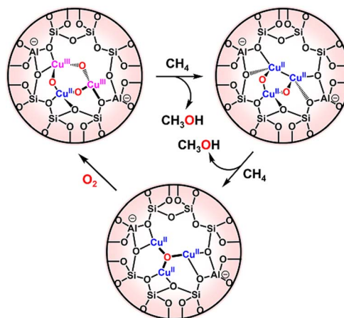
Fig. 16 Formation of a [Cu 3 (μ 3 -O)] 2+ species and two CH 3 OH molecules from the reaction of CH 4 with [Cu 3 (μ-O)] 2+ in MOR zeolite. Adapted from ref. 252.
