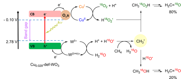
Fig. 21 Proposed mechanism for charge transfer steps during selective CH_4 oxidation over Cu_{0.029}\text{-def-}WO_3 .
