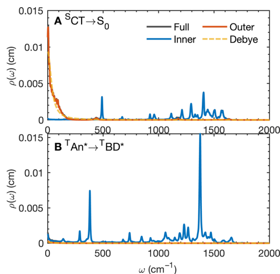
Fig. 4 Spectral distribution \rho(\omega) for (A) the {}^{\text{S}}\text{CT} \rightarrow \text{S}_0 process computed from dynamics on the {}^{\text{S}}\text{CT} potential energy surface and (B) the {}^{\text{T}}\text{AN}^* \rightarrow \text{T}^{\text{BD}}^* process computed from dynamics on the {}^{\text{T}}\text{AN}^* potential energy surface. The decomposition into inner and outer sphere contributions and the Debye approximation for the outer-sphere component is also shown, \rho_{\text{D}}(\omega) = (2/\pi)/(1 + \tau_{\text{D}}^2\omega^2) , where \tau_{\text{D}} = (\epsilon_{\infty}/\epsilon_r)\tau_{\text{rel}} , and \tau_{\text{rel}} is the solvent dipole-dipole autocorrelation relaxation time, and \epsilon_{\infty}/\epsilon_r are the optical and static dielectric constants of the ACN model.
