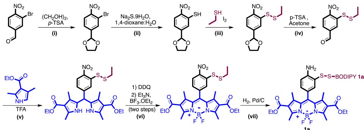
Scheme 1 The synthesis of probe 1a with 2-aminothiophenol reactive core and BODIPY for fluorescence. (i) Toluene, 60 °C, 6 h, 97%; (ii) 1,4-dioxane, water (2 : 1), 0 °C → rt, 20 h, 75%; (iii) DMSO, 50 °C, 7 h, 76%; (iv) acetone, reflux, 7 h, 56%; (v) DCM, rt, 5 h, 92%; (vi) DCM, 0 °C → rt, 5 h, 72%; (vii) DCM, rt, 5 h, 46%.
