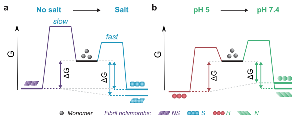
Fig. 5 Schematic representation of energy landscapes of the different types of \alpha Syn fibrils studied. Effect of (a) salt and (b) pH on the kinetics of formation and stability of fibrils. Different fibril polymorphs are depicted by different shapes of their monomer building blocks (NS – triangles, S – squares, H – circles, N – parallelograms) and color-coded according to the conditions they were formed (NS – violet, S – blue, H – red, N – green). A change in solution conditions can both increase (a) and decrease (b) the thermodynamic stability of a given type of fibril.
