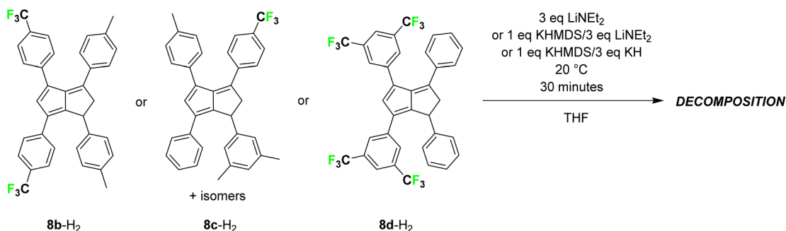
Scheme 4 Attempted deprotonative metalations of (\text{CF}_3)_x\text{Ph} -substituted dihydropentalenes 8b-H 2 , 8c-H 2 and 8d-H 2 ( x = 1 or 2 ).
