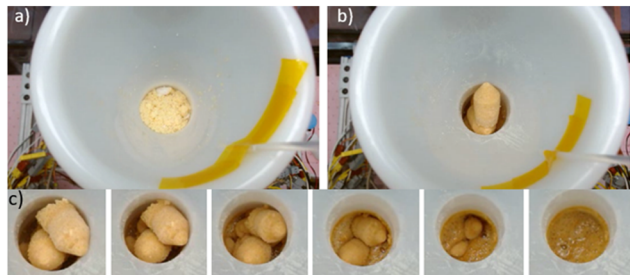
Fig. 11 a) Overhead view of the plate reactor feed hopper with loose powder. b) Feed hopper with powder plugs formed in conical vials. c) Time-lapse view of the powder plugs traveling down the feed hopper and melting.
