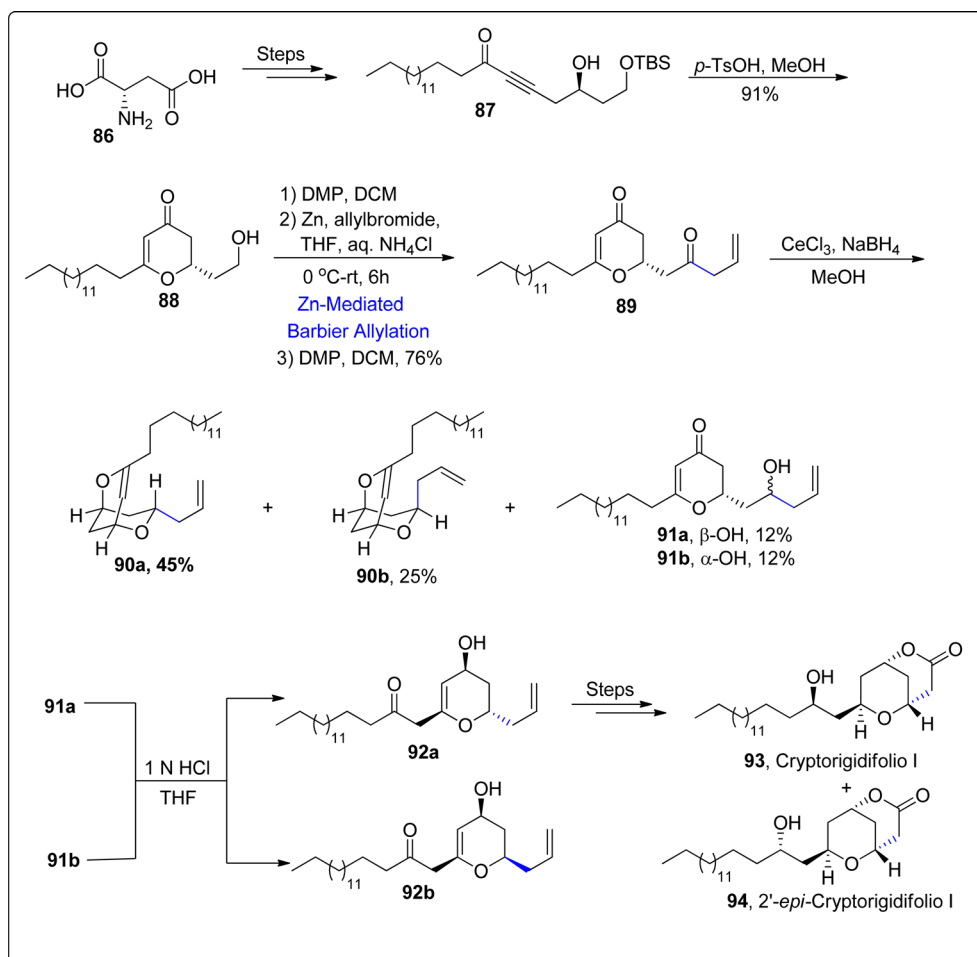
Scheme 12 Synthesis of cryptorigidifoliol 93 and 2'- epi -cryptorigidifoliol 94 .
