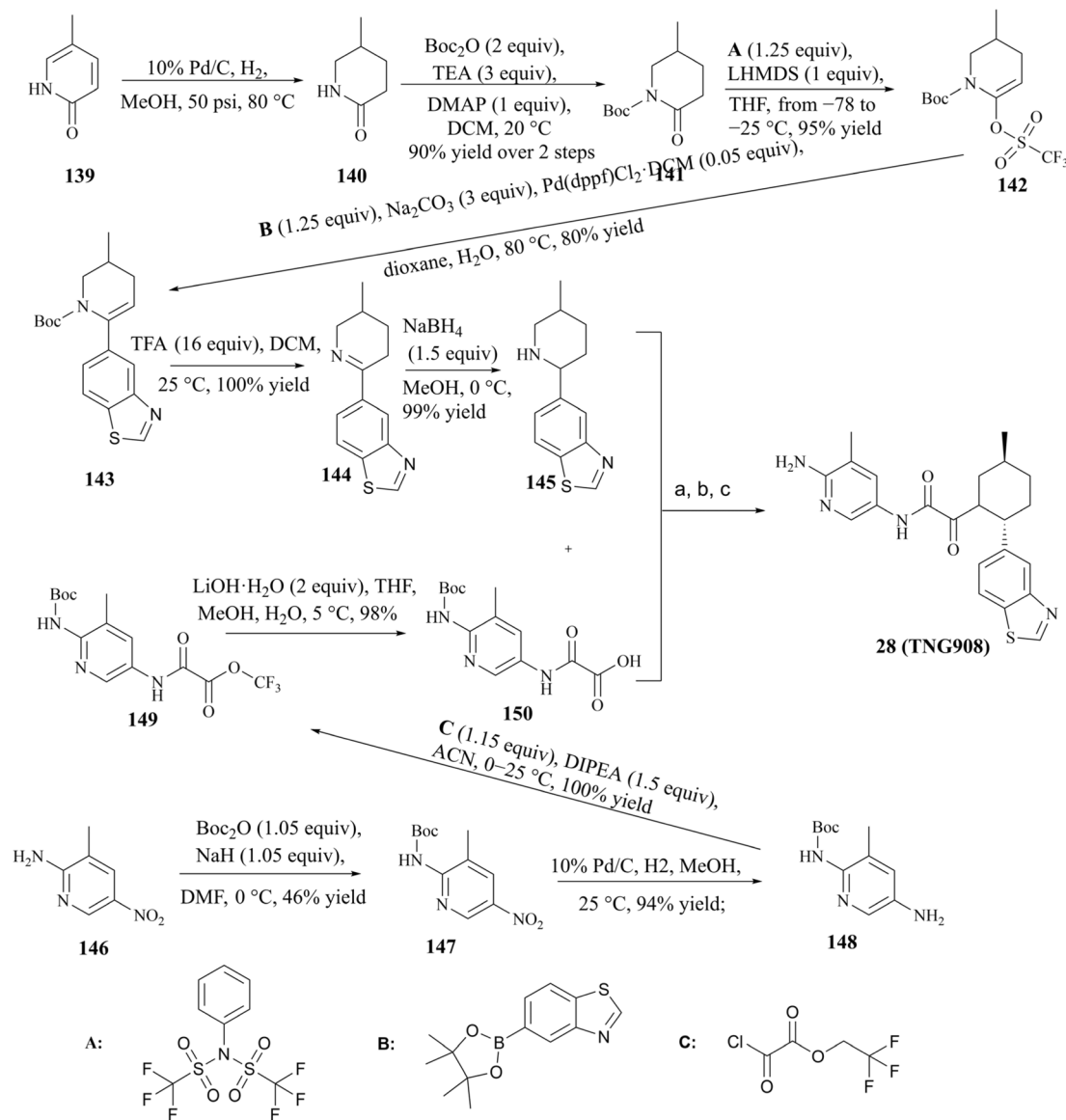
Fig. 26 28 (TNG908) preparation route. (a) HATU (1 equiv.), TEA (6 equiv.), DMF, 25 ^{\circ}\text{C} ; (b) 4 M HCl in dioxane, 25 ^{\circ}\text{C} , 59% yield over 2 steps for 28 (TNG908); (c) chiral HPLC separation of enantiomers, 48% yield for 28 (TNG908).
