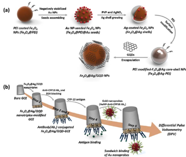
Fig. 14 Synthesis of \text{Fe}_3\text{O}_4@Ag/GQD NP nanotriplex (a) immunosensor preparation (b): drop casting onto the GCE (step 1), incubation with CAB (step 2), blocking with BSA (step 3), incubation with the target antigen (step 4), and incubation with the AbD-AuNPs (step 5). Reprinted with permission from ref. 232. Copyright © 2018 Elsevier Ltd.
