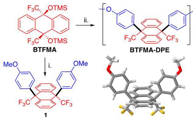
Fig. 2 Synthesis of model compound 1 , shown with its single crystal XRD structure (CCDC 2382285†) confirming its “cis” configuration of substituents relative to the anthracene plane, and polymer BTFMA-DPE . Reagents and conditions: i. anisole, TFSA, DCM, 20 °C; ii. DPE, TFSA, DCM, 20 °C (90% yield).
