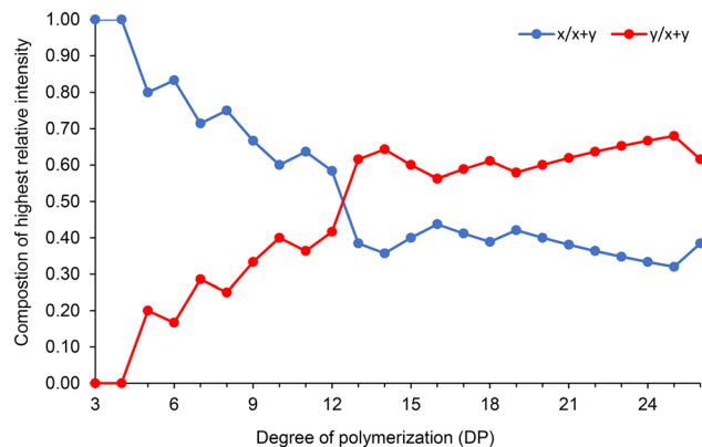
Fig. 8 Variation of the composition ( x, y ) in P[(\text{CL}^{\text{nBu}})_x\text{-co-(CL}^{\text{Me}})_y] copolymers as a function of the degree of polymerization (DP). The composition was calculated from the most intense m/z signal for a defined DP, from MALDI-ToF MS of P(\text{CL}^{\text{nBu}}\text{-co-CL}^{\text{Me}}) copolymers prepared by the ROCOP of a 1 : 1 mixture of ( R )- \text{CL}^{\text{nBu}} and ( S )- \text{CL}^{\text{Me}} with the 1a /BnOH catalytic system, over 35 min (Table 1, entry 1).
