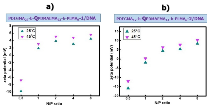
Fig. 6 Zeta-potential values vs. N/P ratios for PDEGMA 23 - b -QPDMAEMA 23 - b -PLMA 8 -1/DNA (a) and PDEGMA 17 - b -QPDMAEMA 14 - b -PLMA 6 -2/DNA (b) micelleplexes at 25 °C and 45 °C.
