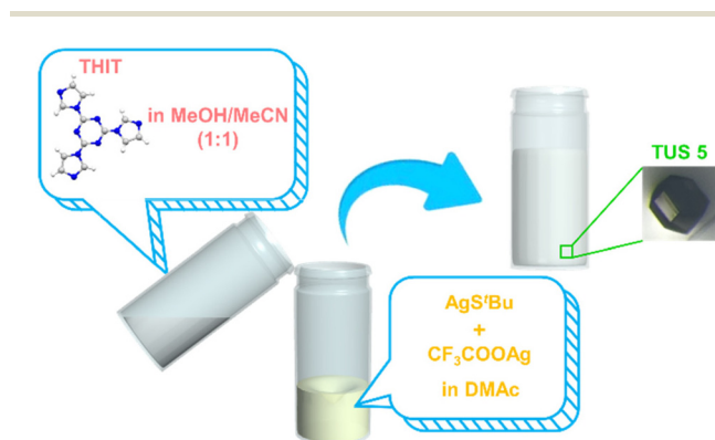
Fig. 1 Schematic diagram portraying the synthesis procedure of TUS 5 single crystals. The magnified view of the bottom surface of the product vial displays the optical microscopy image of the single crystal. Color scheme: N, blue; C, grey; and H, white.
