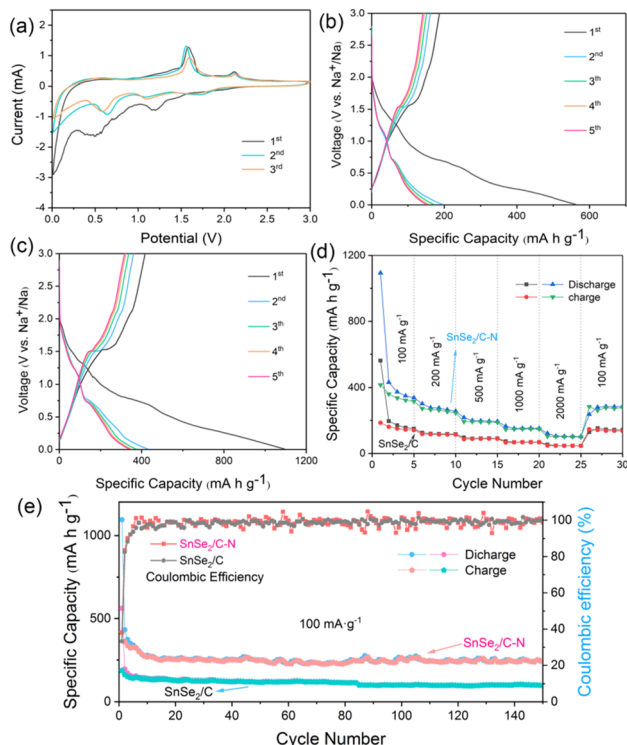
Fig. 5 (a) CV curves of \text{SnSe}_2/\text{C-N} at 0.1 \text{ mV s}^{-1} ; constant current charge/discharge curves of (b) \text{SnSe}_2/\text{C} and (c) \text{SnSe}_2/\text{C-N} at 0.1 \text{ A g}^{-1} ; (d) rate performance of \text{SnSe}_2/\text{C} , and \text{SnSe}_2/\text{C-N} electrodes at different rates; and (e) cycling performance at 0.1 \text{ A g}^{-1} .
