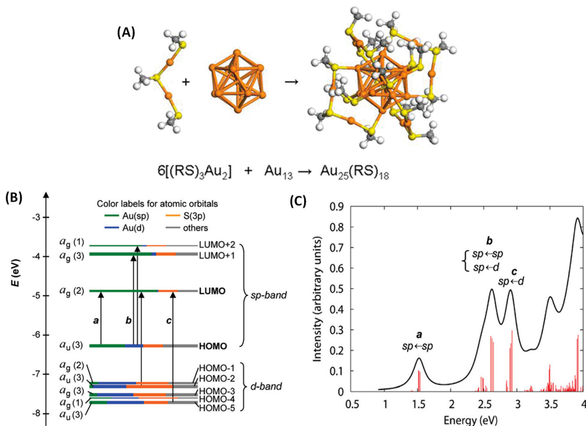
Fig. 2 (A) Schematic of the crystal structure of \text{Au}_{25}(\text{SR})_{18} ( -\text{SR} = alkyl/aryl thiolate), which consists of six \text{Au}_2(\text{SR})_3 staple motifs protecting an \text{Au}_{13} icosahedral core. Color code: orange (Au) and yellow (S). (B) Kohn–Sham orbital energy level diagram for \text{Au}_{25}(\text{SH})_{18}^- . The energies are in units of eV. Each KS orbital is drawn to indicate the relative contributions (line length with color labels) of the atomic orbitals of Au (6sp) in green, Au (5d) in blue, S (3p) in yellow, and others in gray (those unspecified atomic orbitals, each with a <1% contribution). The left-hand column of the KS orbitals shows the orbital symmetry (g, u) and degeneracy (in parentheses); the right-hand column shows the HOMO and LUMO sets. (C) The theoretical absorption spectrum of \text{Au}_{25}(\text{SH})_{18}^- . Peak assignments: peak a corresponds to 1.8 eV observed, peak b corresponds to 2.75 eV (observed), and peak c corresponds to 3.1 eV (observed). (A) is reproduced from ref. 34a with permission from the American Chemical Society, Copyright 2008; B and C are reproduced from ref. 34b with permission from the American Chemical Society, Copyright 2008).
