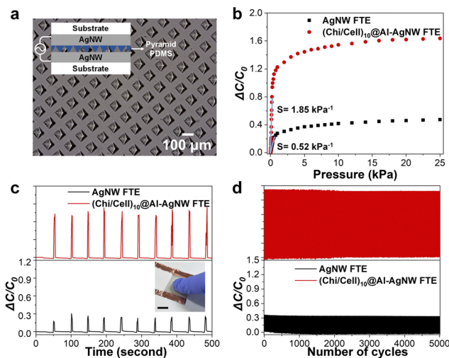
Fig. 6 (a) Optical image of the micropatterned PDMS elastomer inserted between FTEs. The inset in (a) shows the schematic of the pressure sensor. (b) Relative capacitance change ( \Delta C/C_0 ) and sensitivity of pressure sensors composed of AgNW and (Chi/Cell) 10 @Al-AgNW FTEs as a function of pressure. Relative capacitance change ( \Delta C/C_0 ) of the pressure sensors composed of AgNW and (Chi/Cell) 10 @Al-AgNW FTEs as a function of time with (c) gentle finger touch and (d) repeated loading–unloading cycles at a fixed pressure of 2.5 kPa. The inset in (c) shows the photograph of a gentle finger touch, and the scale bar represents 1 cm.
