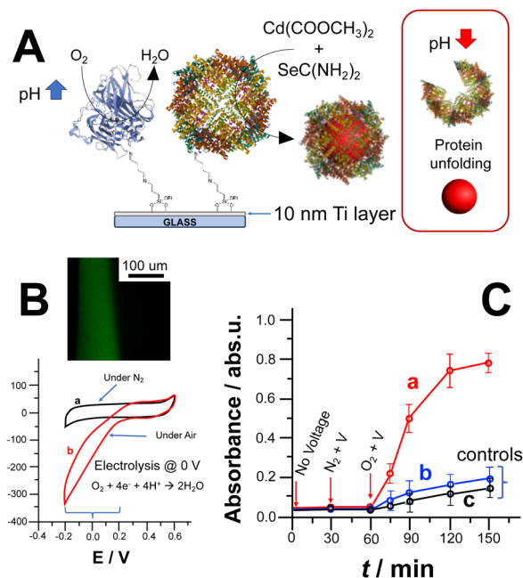
Fig. 2 (A) Scheme reporting Ti electrode modified with laccase/apoferritin, notably as pH shift trigger and bionanoreactor, and CdSe NPs synthesis upon pH shift due to ORR followed by particles release; (B) cyclic voltammograms recorded with the \text{TiO}_2 modified electrode with ferritin and laccase ( 1 \text{ cm}^2 geometrical area) with the absence (a) and presence of \text{O}_2 (in equilibrium with air). Potential scan rate, 5 \text{ mV s}^{-1} . Background electrolyte: \text{NH}_3/\text{acetate} buffer (3 mM, pH 6.5 containing 0.1 M \text{Na}_2\text{SO}_4 ) – inset: CFM image of pH gradient at the electrode surface; (C) UV-Vis kinetics measurements of reaction media after applying 0 \text{ V vs. Ag/AgCl} for (a) CdSe NPs synthesis upon local pH change induced by ORR catalysed by laccase, (b) control experiment for CdSe NPs synthesis without laccase performed applying 0 \text{ V vs. Ag/AgCl} and (c) control experiment without applying any voltage.
