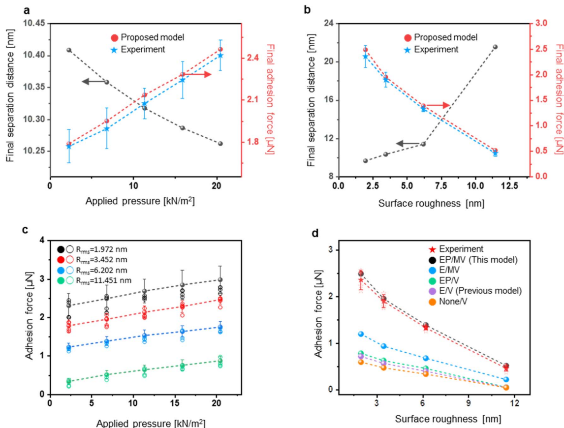
Fig. 6 Experimental verification of Mo–Mo contact (metallic contact): (a) graph of the final separation distance (left axis) and the final adhesion force (right axis) versus applied pressure for the sample having a surface RMS roughness of 3.452 nm. (b) Graph of the final separation distance (left axis) and the final adhesion force versus surface RMS roughness under the applied pressure of 6.81 \text{ kN m}^{-2} . The red circles on the right axis present the predicted values of the adhesion forces obtained utilizing the proposed model, and the blue stars present the experimental value of the adhesion forces obtained from the AFM F – d experiment. (c) Quantitative comparison between the predicted (filled) and experimental (open) values of the adhesion forces according to various contact forces applied to the surface having RMS roughness of 1.972 nm, 3.452 nm, 6.202 nm, and 11.451 nm. (d) Comparison between the experimental and predicted values of the adhesion forces at the applied external force of 300 \mu\text{N} when different models were used. Different combinations of deformation regions (E: elastic deformation, P: plastic deformation) and intermolecular forces (V: van der Waals force, M: metallic bonding force) were considered for each model. The red stars represent the experimental values. The black circles are the computed values obtained from the proposed contact model by considering both elastic and plastic deformations, and both metallic bonding and van der Waals forces. The blue circles are also computed values using the proposed model when only elastic deformation was considered along with the metallic bonding and van der Waals forces. Lastly, the green, purple, and orange represent the computed values, in which metallic bonding forces were not considered as part of the calculations. However, all deformation regions were considered for the data represented in the green circles while only the elastic deformation region accounted for those shown in purple. Lastly, the data shown in orange represents the computed adhesion forces when mechanical deformation of the asperities was factored out.
