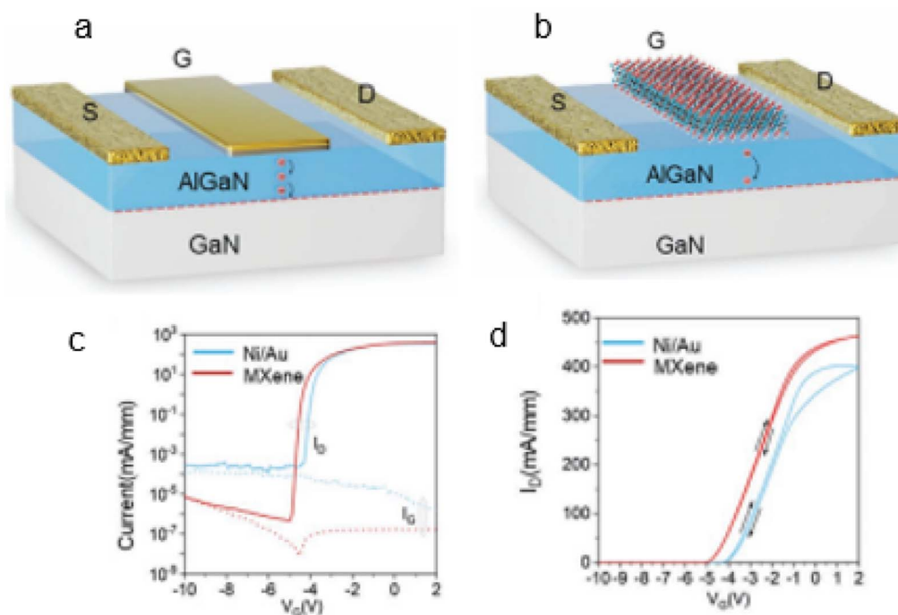
Fig. 18 GaN HEMT schematic diagrams with either Ti 3 C 2 T x or (a) Ni/Au or (b) the gate electrodes. (c) The Ni/Au- and MXene-gate GaN HEMTs' I G curves and logarithmic-scale transfer curves. (d) GaN HEMT dual-sweep transfer curves on a linear scale (copyright 2023 John Wiley and Sons).
