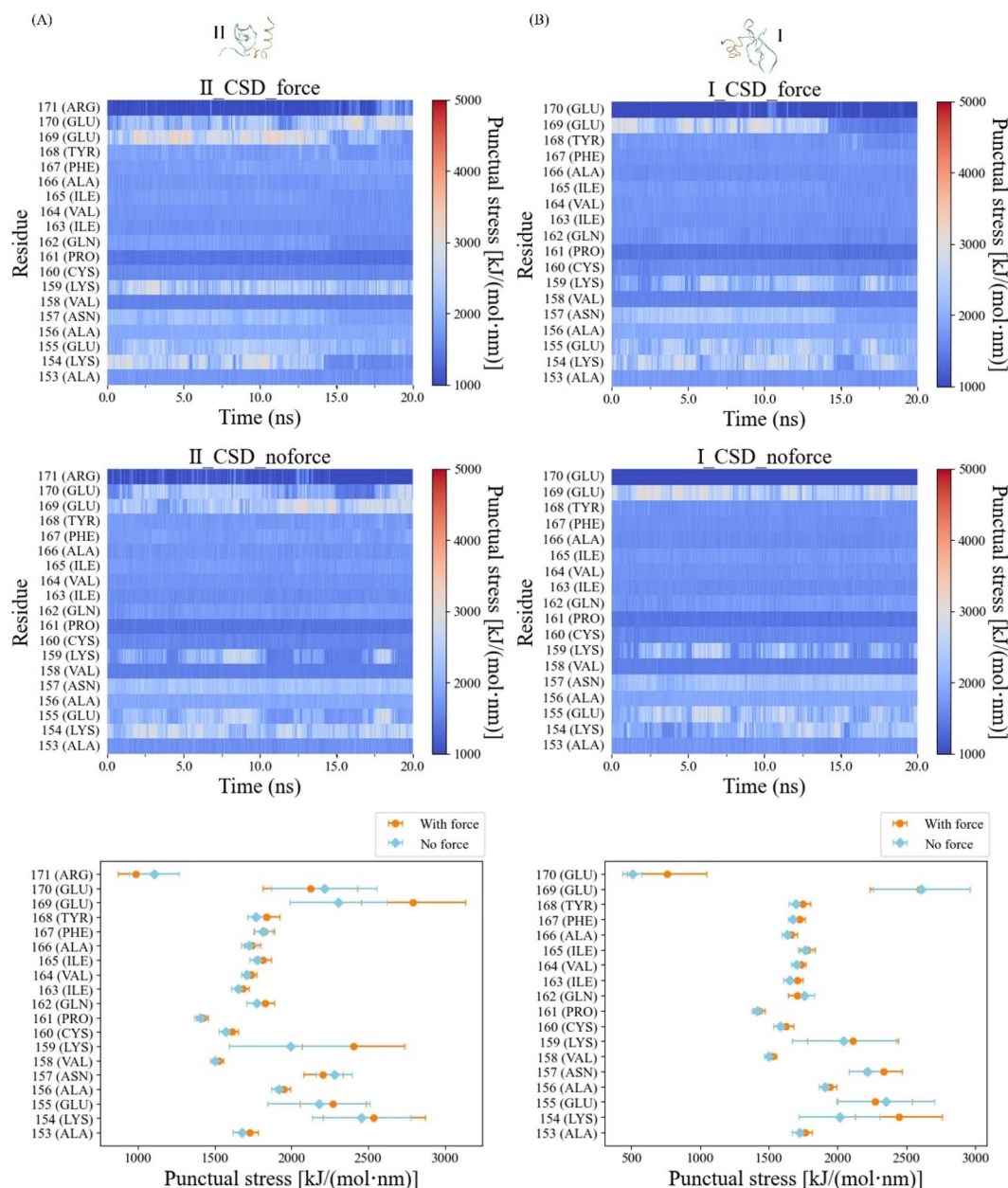
Fig. 6 Force distribution analysis for the (A) constrained 11 CSD monomer (left) and (B) unconstrained 1 CSD monomer (right) along the \alpha -helix interface with/without force over the 20 ns simulation. Punctual stress heatmaps were generated by averaging data from three simulations at each time step for both force and no-force conditions. The bar plots display the average punctual stress distributed across residues with standard deviations, for the data recorded before the bond breakage cutoff of 12.5 ns.
