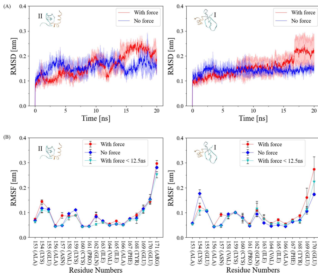
Fig. 3 (A) Root mean square deviation (RMSD) of each \alpha -helix of the ^1\text{CSD} (right, unconstrained) and ^{11}\text{CSD} (left, constrained) throughout the 20 ns simulation, with and without force, and standard deviations indicated by shaded areas. N = 3 for each force and no-force condition. (B) Root mean square fluctuation (RMSF) of each \alpha -helix of the ^1\text{CSD} (right, unconstrained) and ^{11}\text{CSD} (left, constrained) over the 20 ns for both force and no-force conditions, and prior to the 12 ns bond breakage cutoff with force. The results are presented as mean \pm standard deviation. N = 3 for each force and no-force condition.
